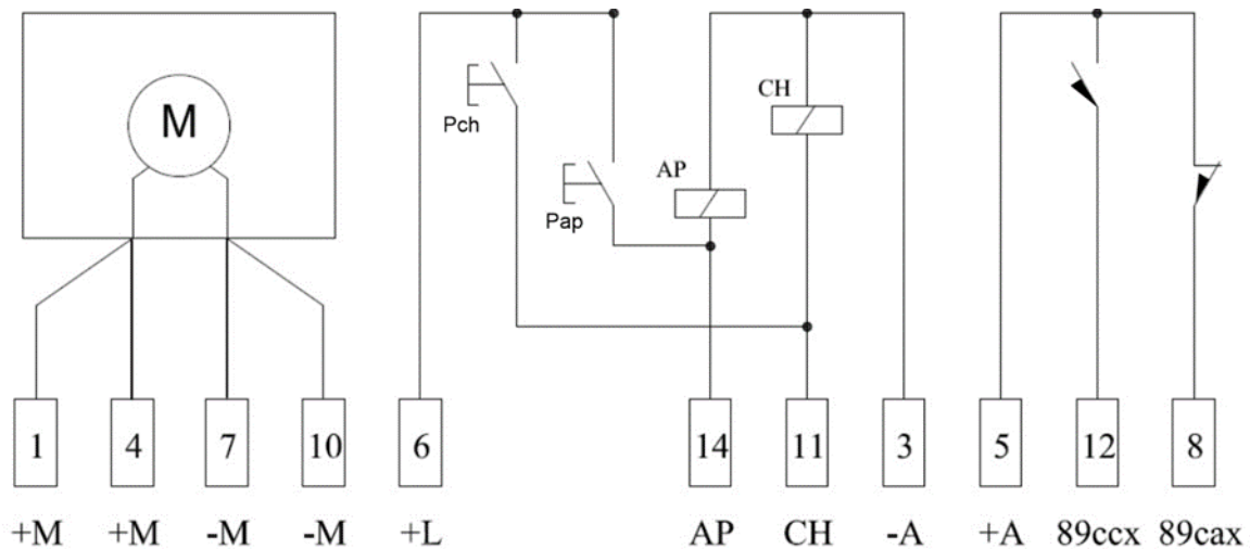
Figure 40 – Electric scheme of switch-disconnector command
