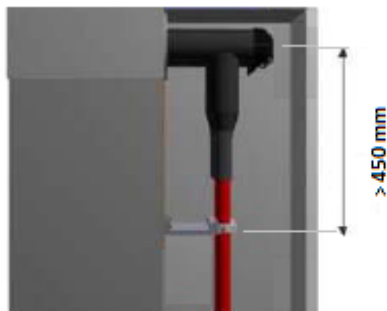
Figure 27 – Examples height of the supports
